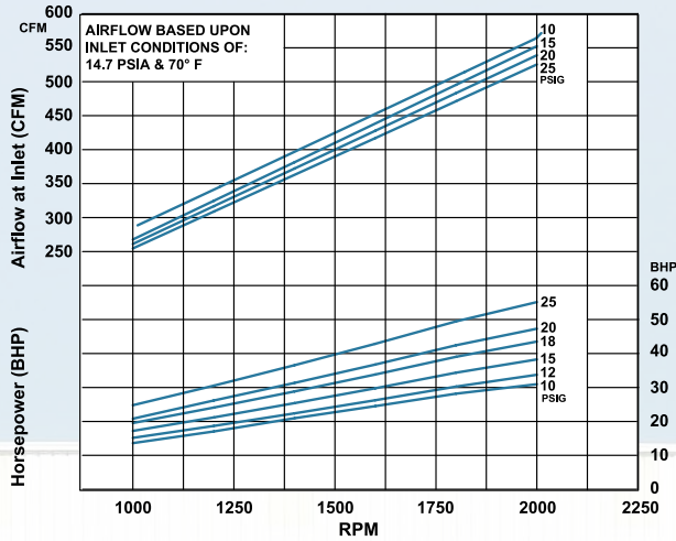
T650 PRESSURE CURVE
