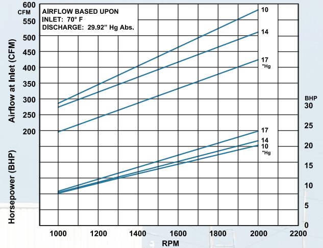
T650 VACUUM CURVE
