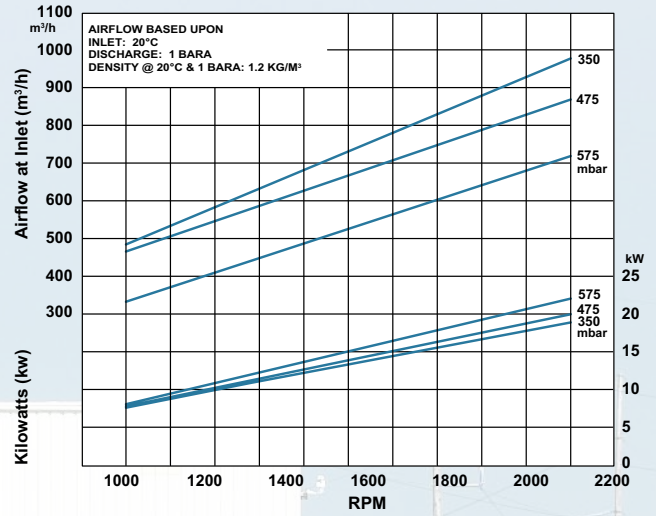
T950H VACUUM CURVE
