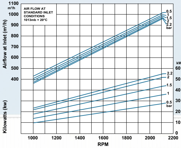
T950H PRESSURE CURVE
